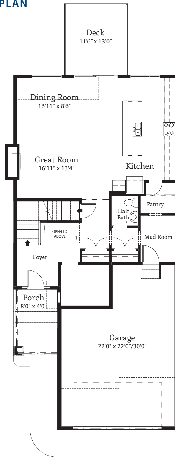
MAIN FLOOR | 1161 sq. ft.
